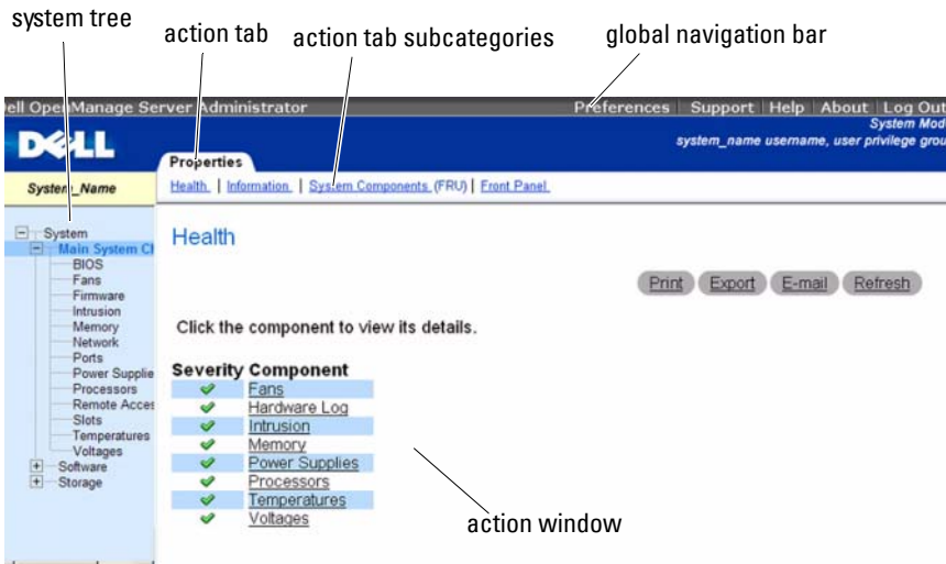
Figure 3-1. Sample Server Administrator Home Page — Non-Modular System
